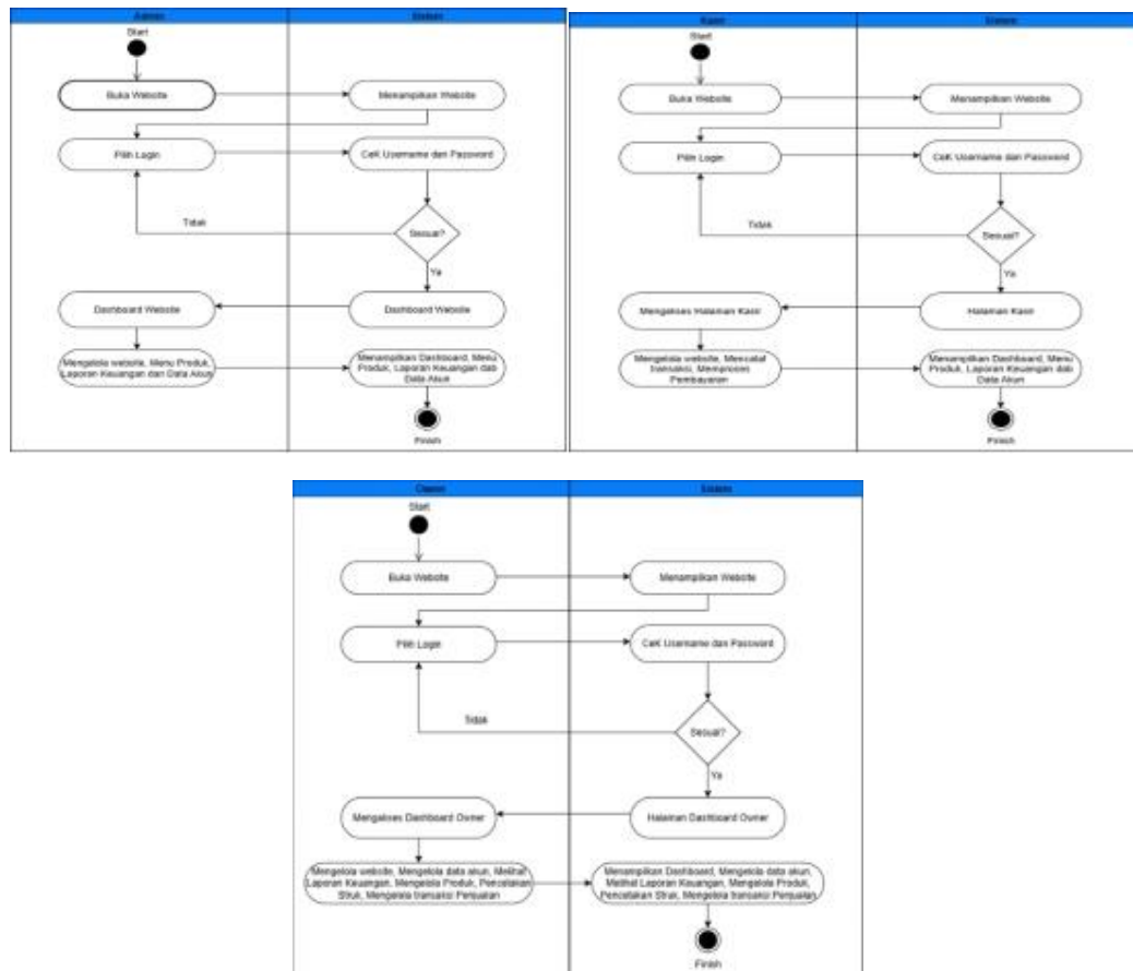
Gambar 3. Activity Diagram
