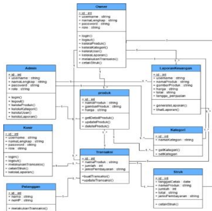
Gambar 4. Class Diagram
