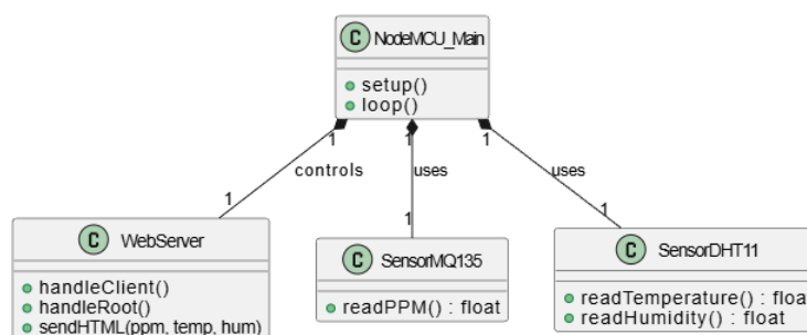
Gambar 3. Class Diagram
