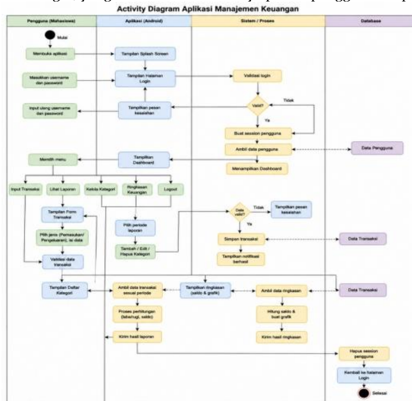
Gambar 3. Activity Diagram
